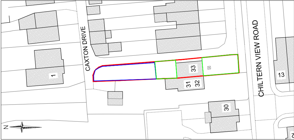
Proposed Site Layout 1:500
