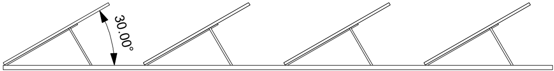
TYPICAL SECTION - 30 DEGREE ANGLE
