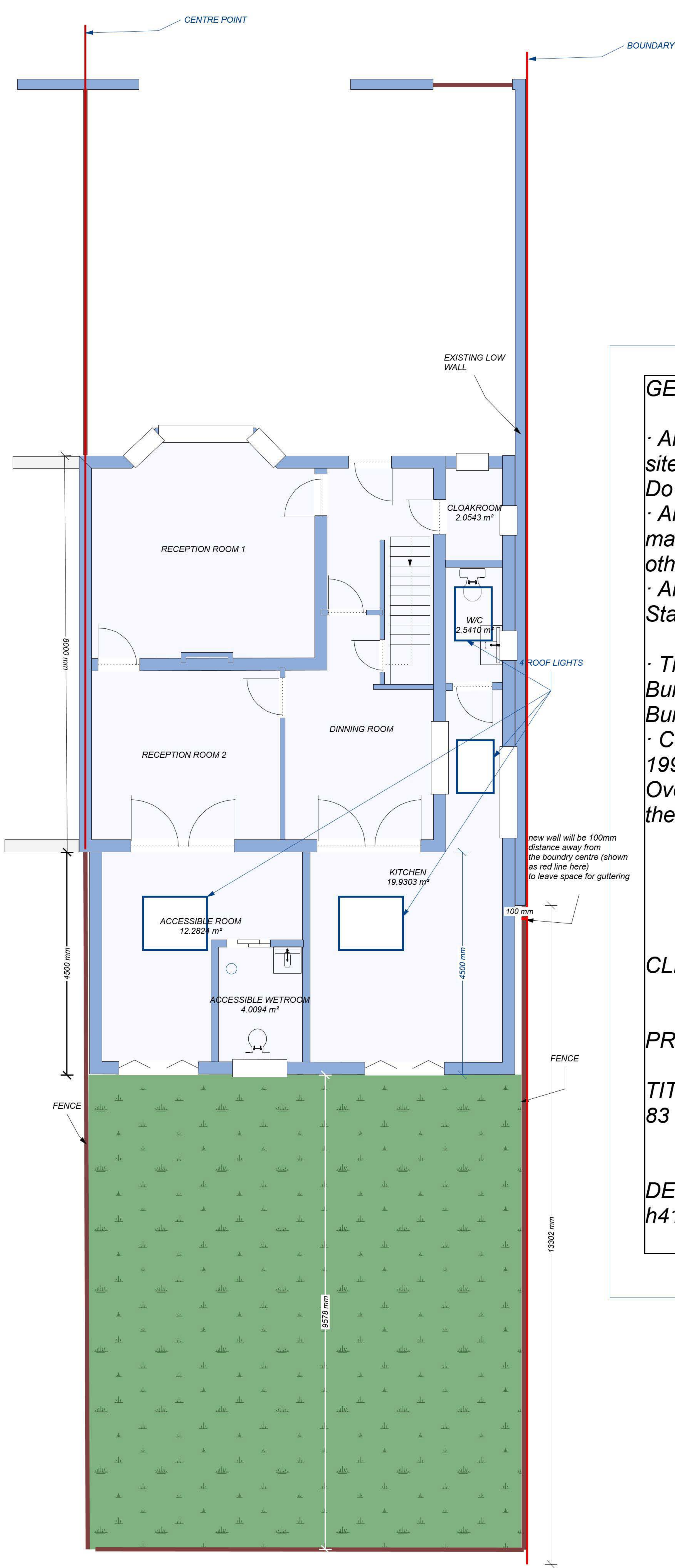
GROUND FLOOR PROPOSED - demolishing the outbuilding & 4.5m rear & side single storey extension
