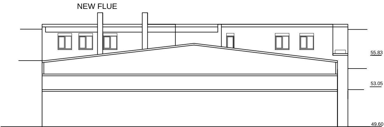
REAR ELEVATION
