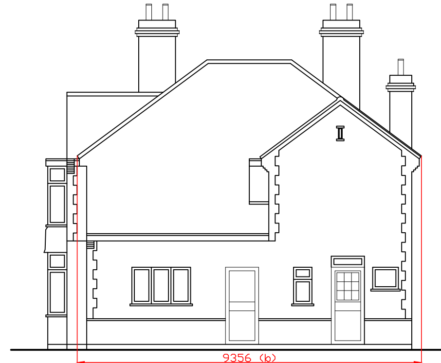
EXISTING SIDE ELEVATION 1
