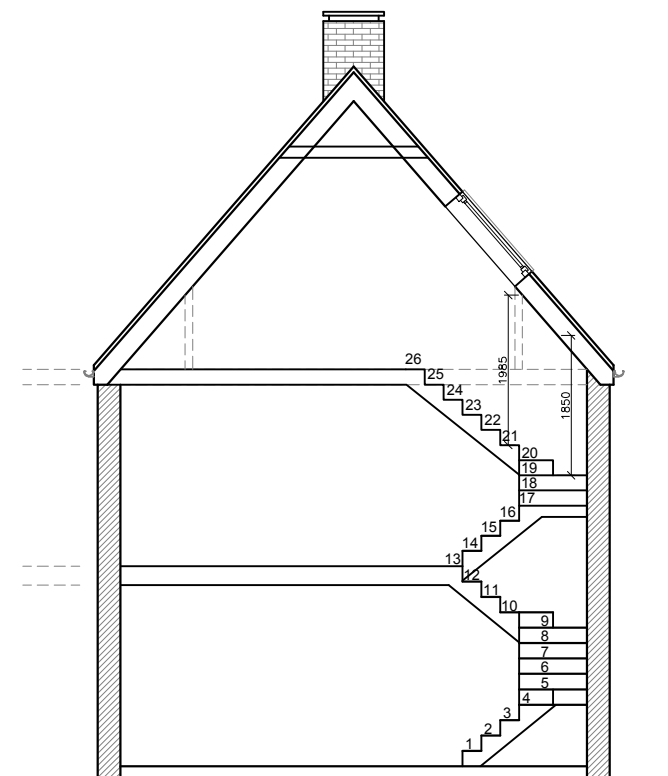
PROPOSED SECTION SCALE= 1:100
