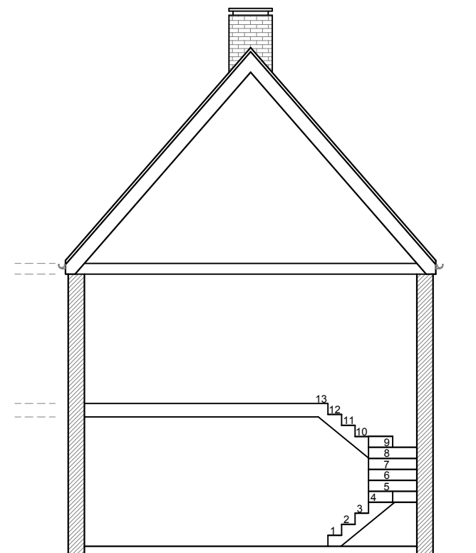
EXISTING SECTION SCALE= 1:100
