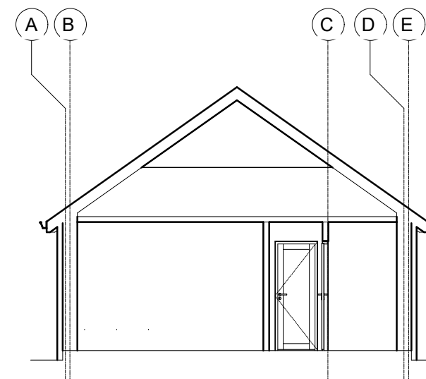
PROPOSED SECTION
