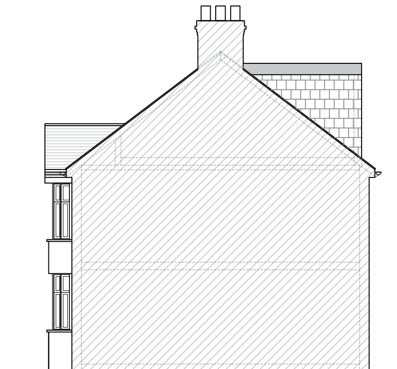
Proposed side elevation (b)
