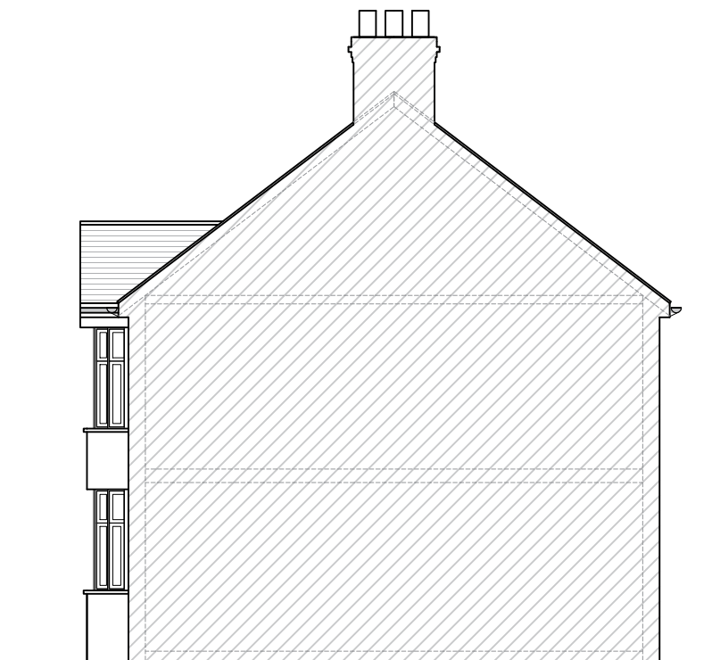
Existing side elevation (b)
