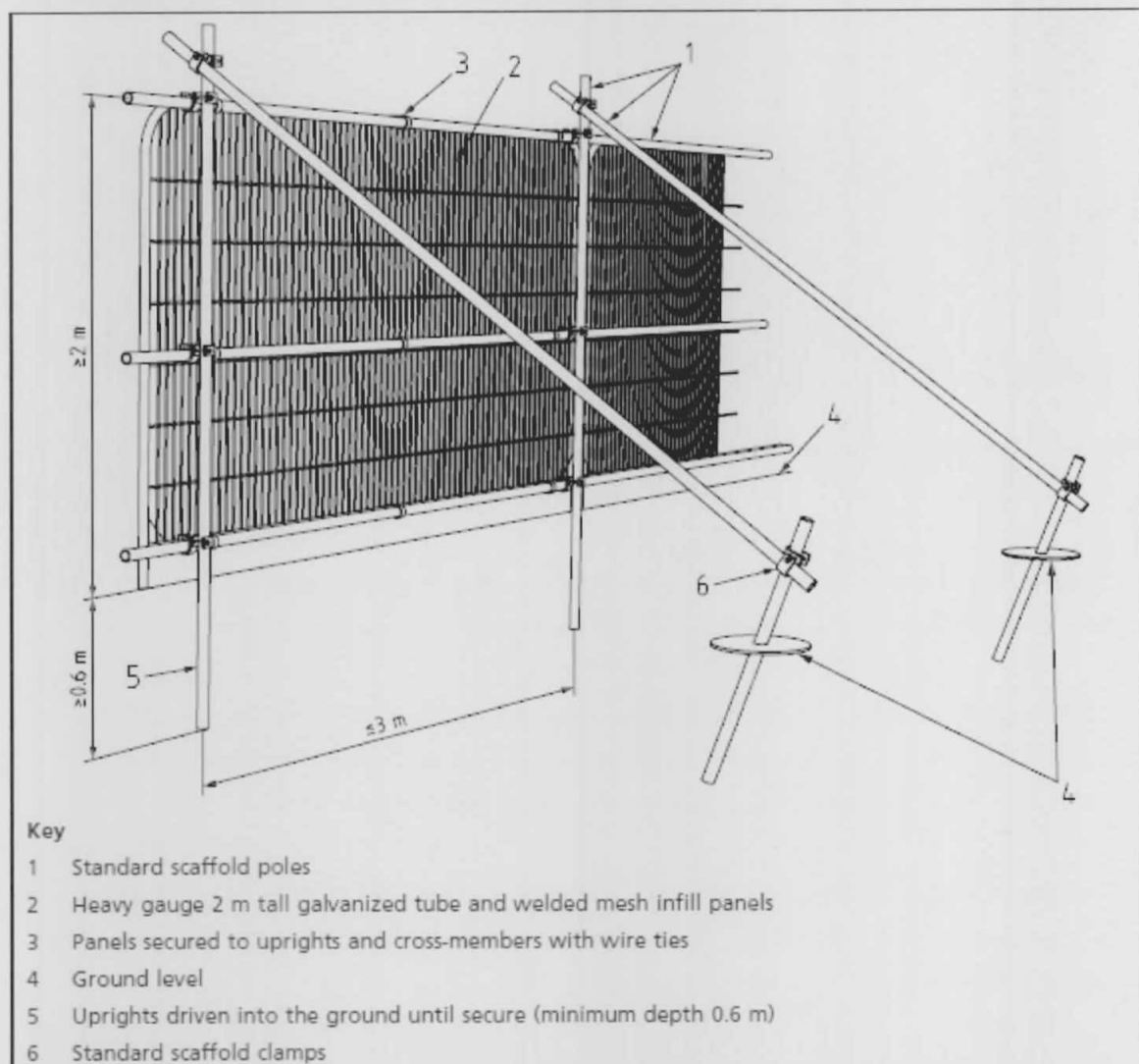
Figure 2: Default specification for protective barrier (BS 5837:2012)
