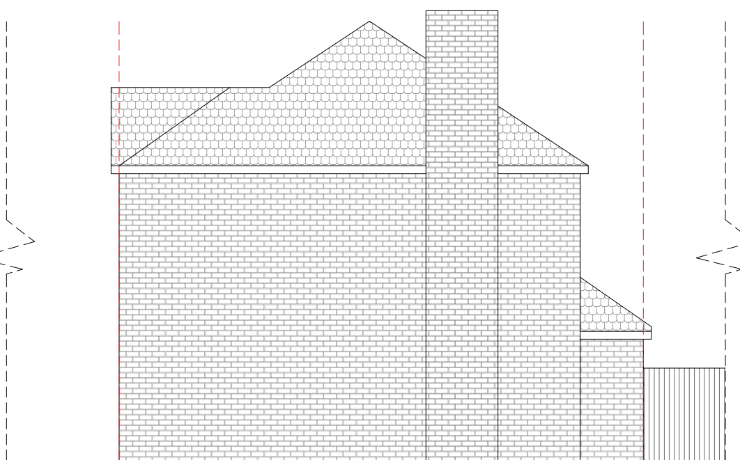
Proposed South Elevation (No Proposed Change)
