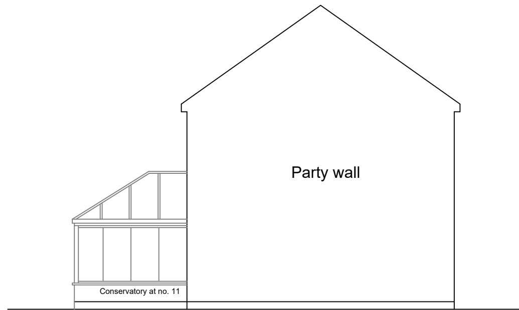
Existing Left Elevation No. 09
