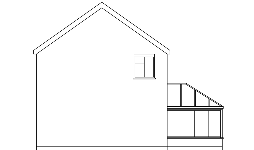
Existing Right Elevation No. 11
