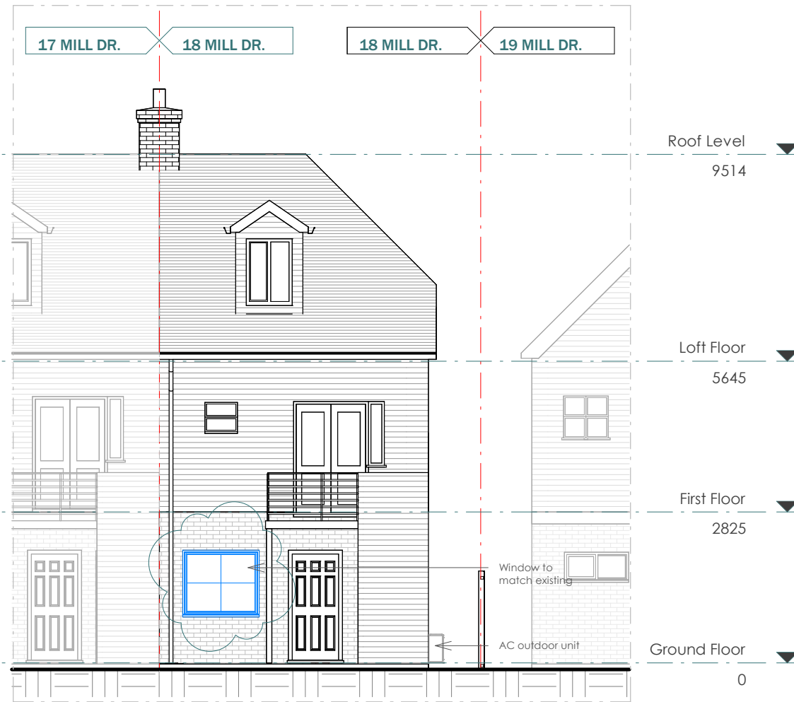
PROPOSED FRONT ELEVATION
