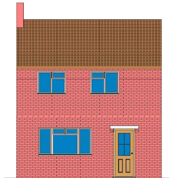
2 Existing Front_Elevation 1 : 100
