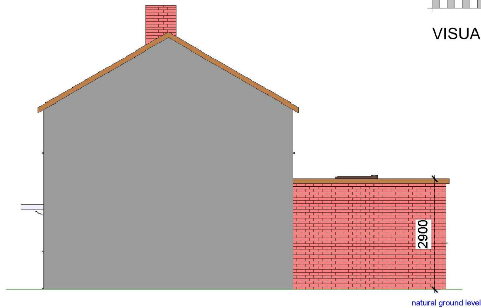
4 Proposed Side 02_Elevation 1 : 100
