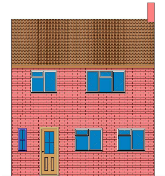
3 Existing Rear_Elevation 1 : 100
