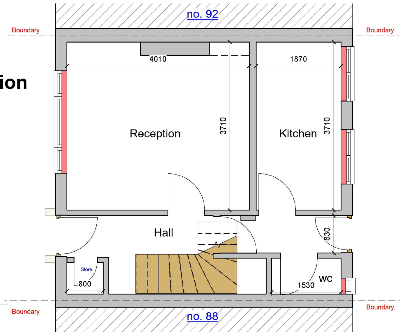
1 Existing Ground Floor 1 : 50
