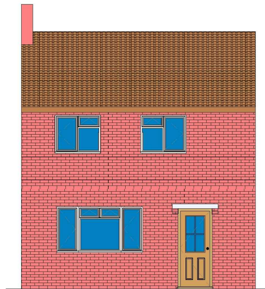
1 Proposed Front_Elevation 1 : 100
