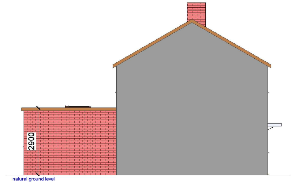
2 Proposed Side 01_Elevation 1 : 100
