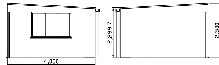
Proposed Side Elevations Scale 1:100
