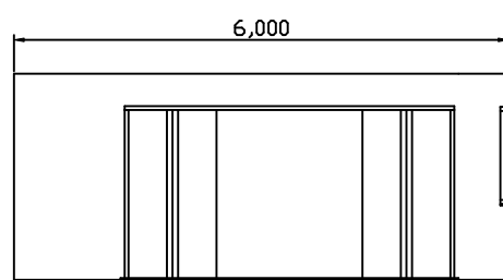
Proposed Front and Rear Elevations Scale 1:100
