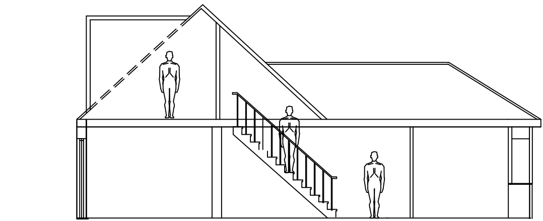
Proposed Cross Plan Scale 1:100
