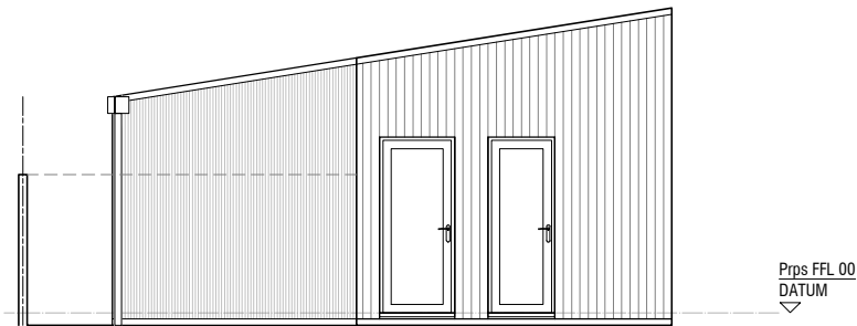
4. PROPOSED SIDE ELEVATION
