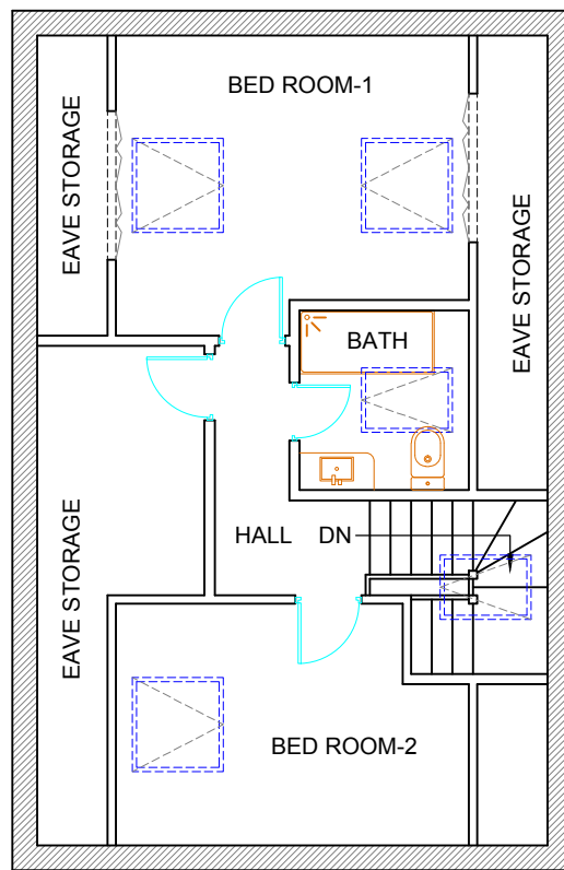
PROPOSED LOFT FLOOR PLAN SCALE= 1:100
