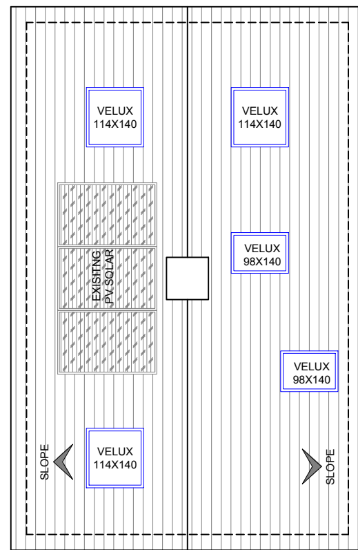
PROPOSED ROOF PLAN SCALE= 1:100
