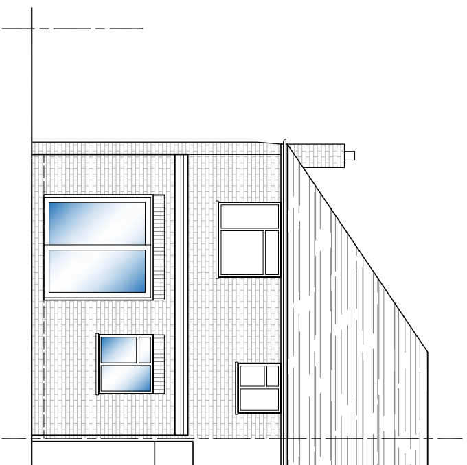
SOUTH ELEVATION
