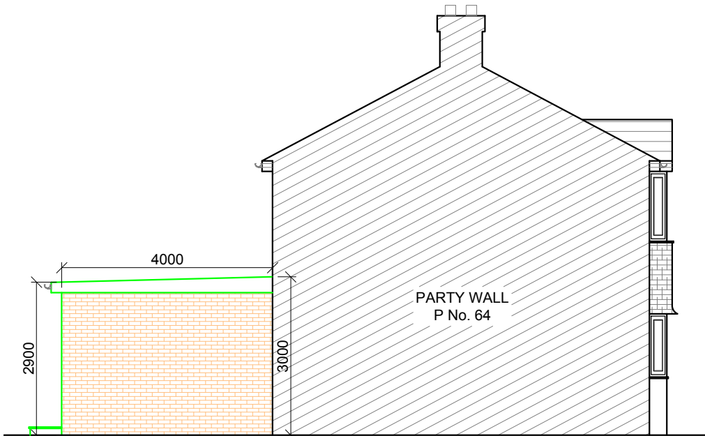
PROPOSED WEST (P-No.64) ELEVATION SCALE= 1:100
