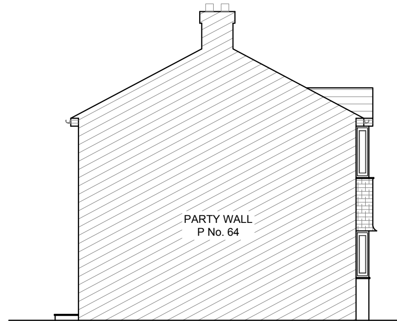
EXISTING WEST (P-No.64) ELEVATION SCALE= 1:100
