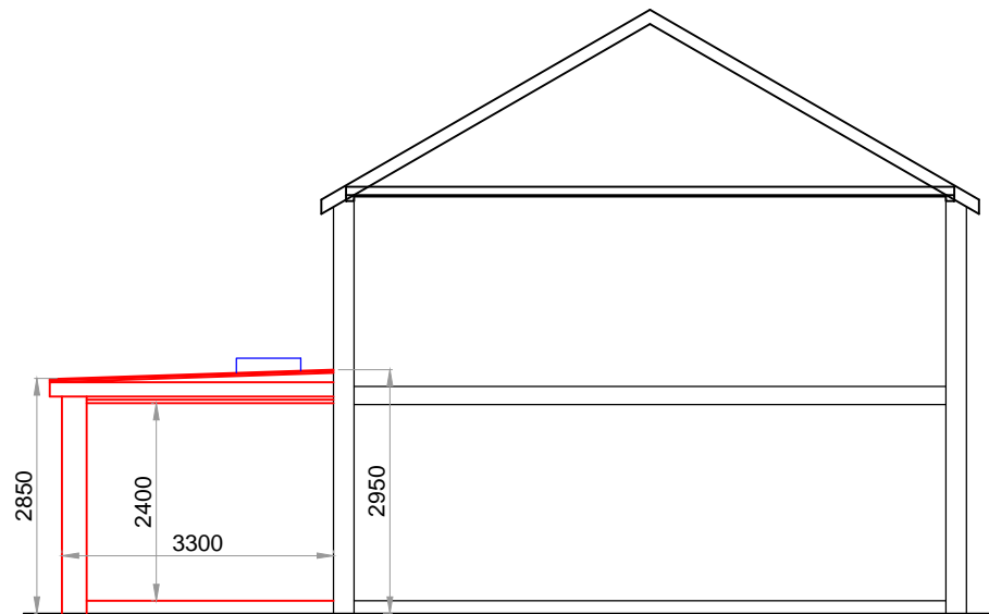
PROPOSED SECTION Scale 1:100
