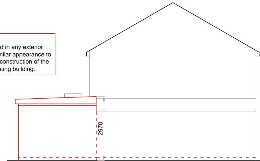
PROPOSED SIDE ELEVATION 02 Scale 1:100
