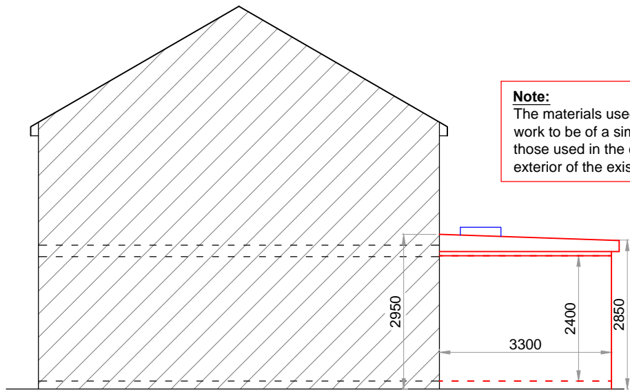
PROPOSED SIDE ELEVATION 01 Scale 1:100
