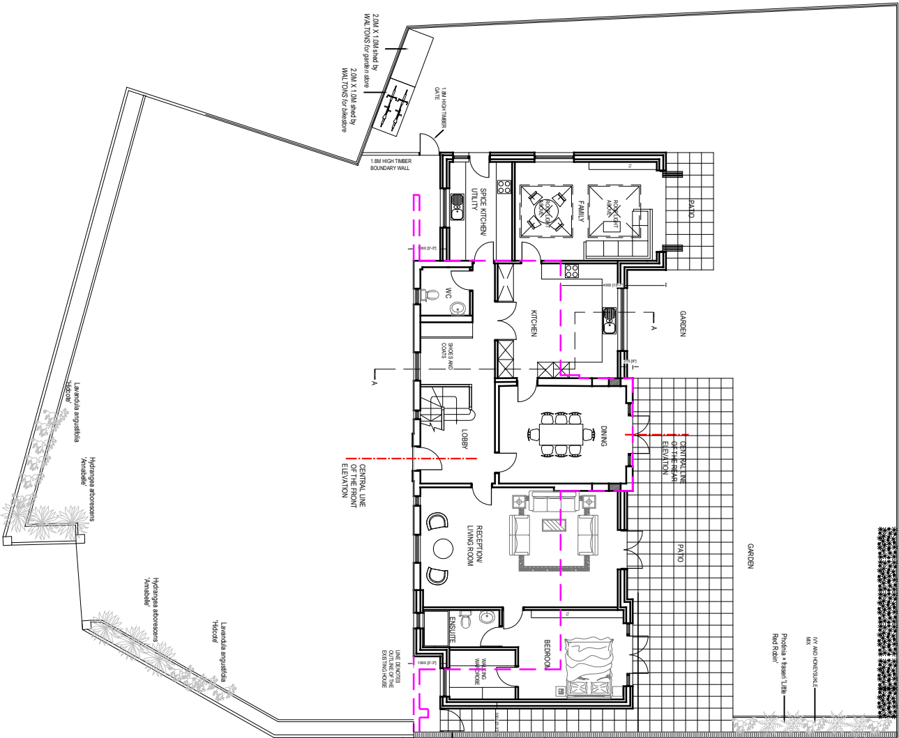
PROPOSED BLOCK PLAN SCALE- 1:200
