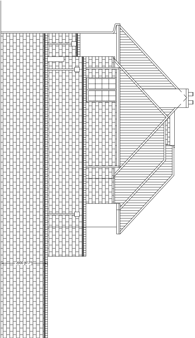
PROPOSED SIDE ELEVATION SHOWING BOUNDARY WALL
