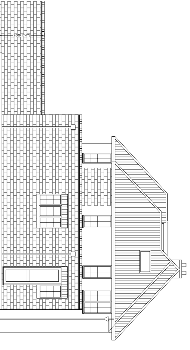
PROPOSED ANOTHER SIDE ELEVATION SHOWING BOUNDARY WALL
