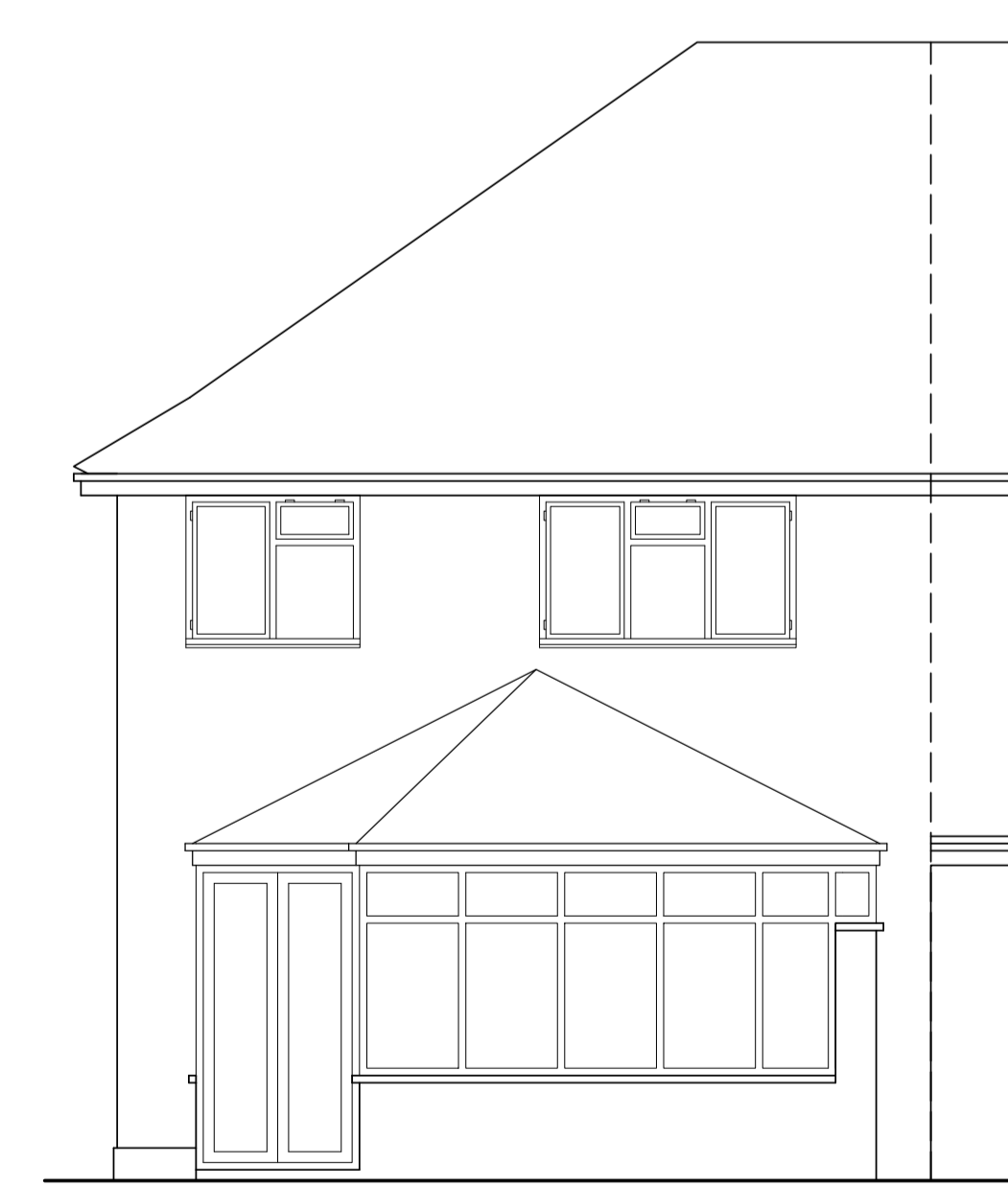
REAR ELEVATION - 1:50
