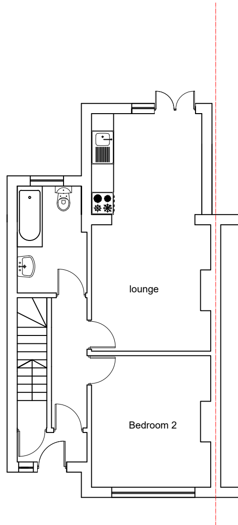
EXISTING AND PROPOSED GROUND FLOOR PLAN
