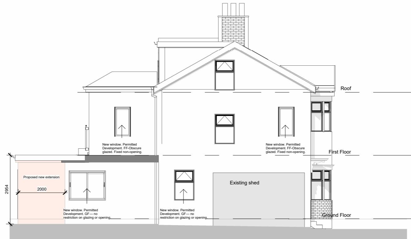
Proposed Left Side Elevation 1:100
