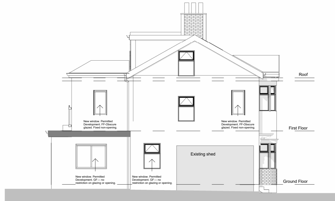
Existing Left Side Elevation 1:100
