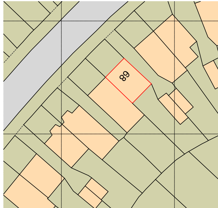
Block plan (1:500)
