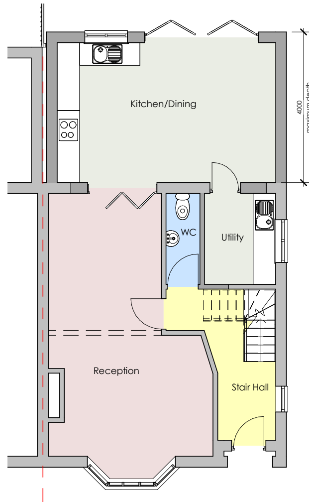
1 Proposed Ground Floor 2553-A-101 1 : 100
