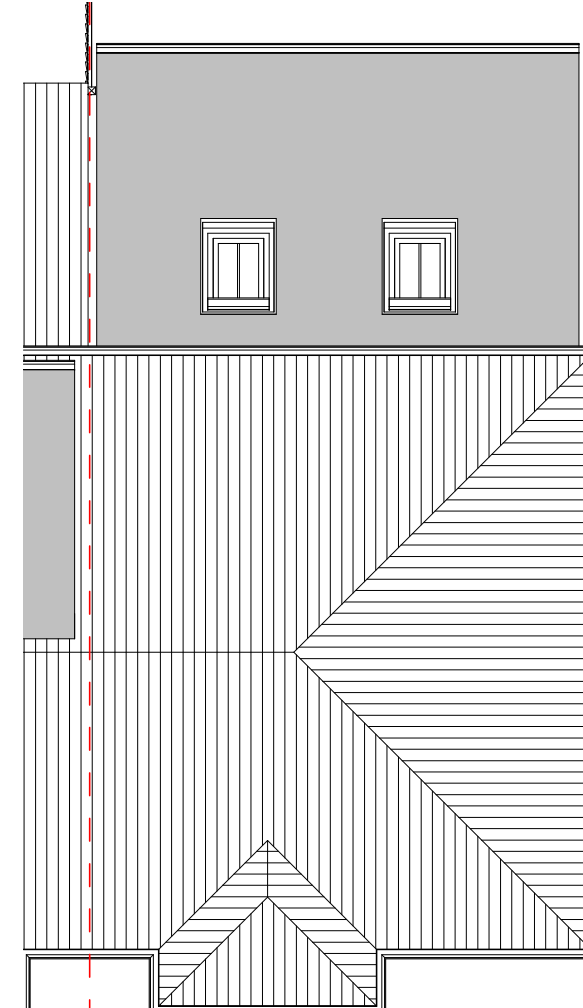
3 Proposed Roof Plan 2553-A-101 1 : 100
