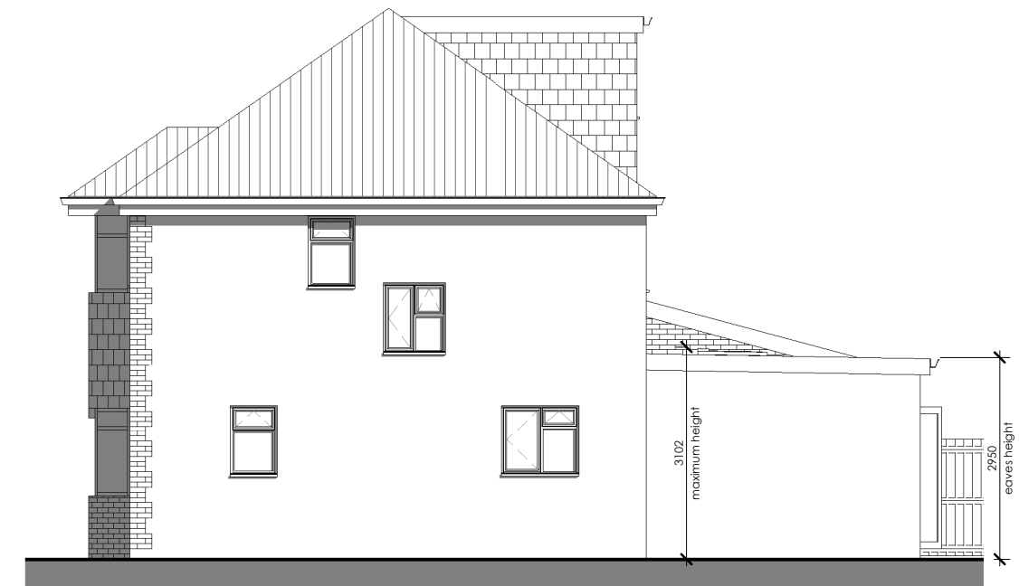
7 Proposed Side Elevation 02 2553-A-101 1 : 100
