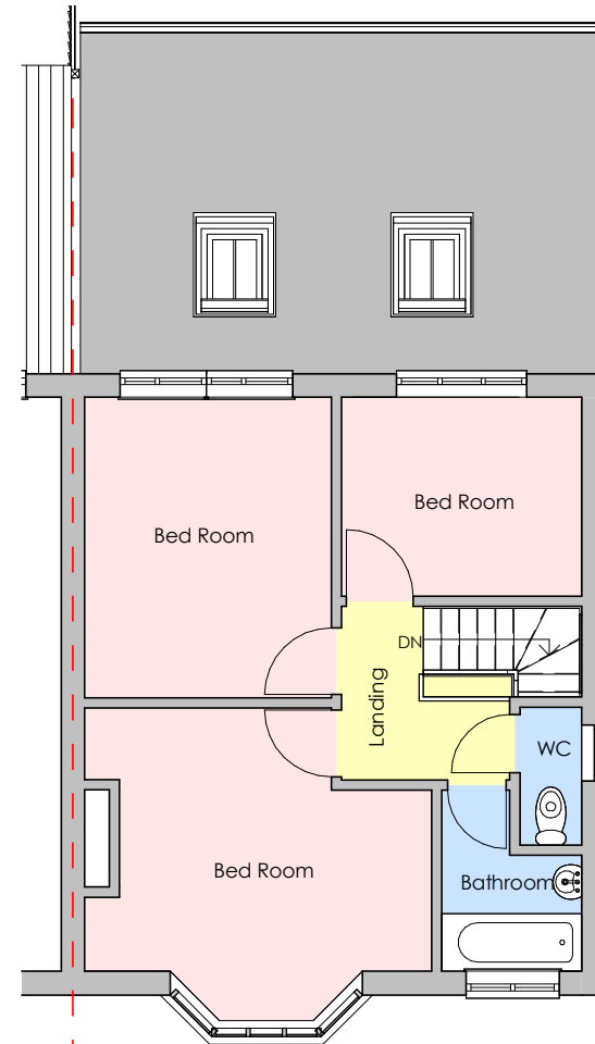
2 Proposed First Floor 2553-A-101 1 : 100
