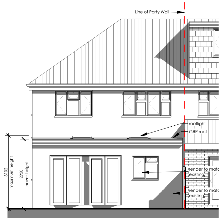
5 Proposed Rear Elevation 2553-A-101 1 : 100
