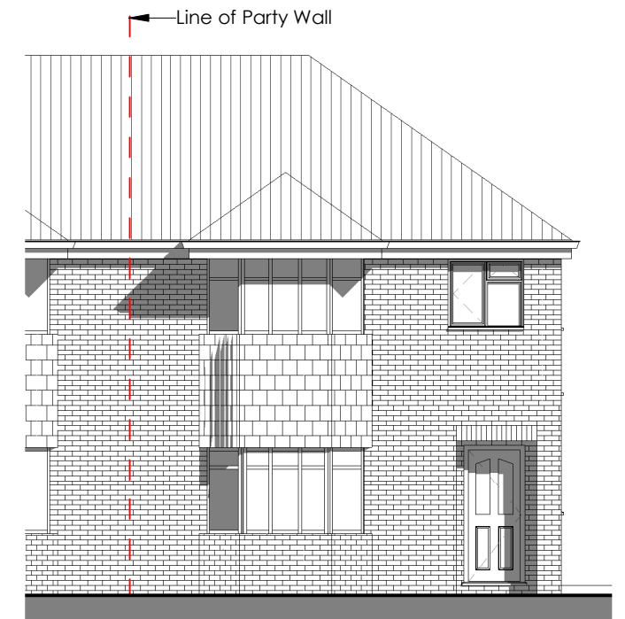
4 Proposed Front Elevation 2553-A-101 1 : 100
