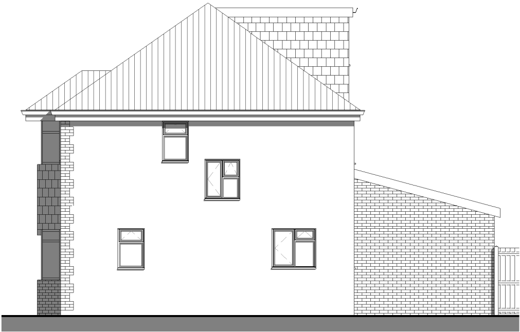
7 Existing Side Elevation 02 2553-A-100 1 : 100
