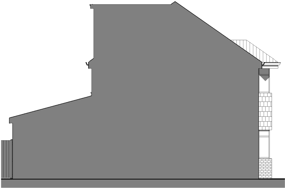
6 Existing Side Elevation 01 2553-A-100 1 : 100
