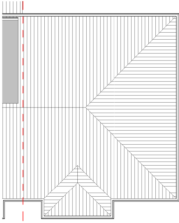
3 Existing Roof Plan 2553-A-100 1 : 100
