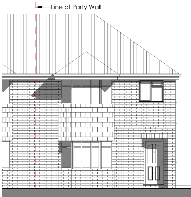
4 Existing Front Elevation 2553-A-100 1 : 100
