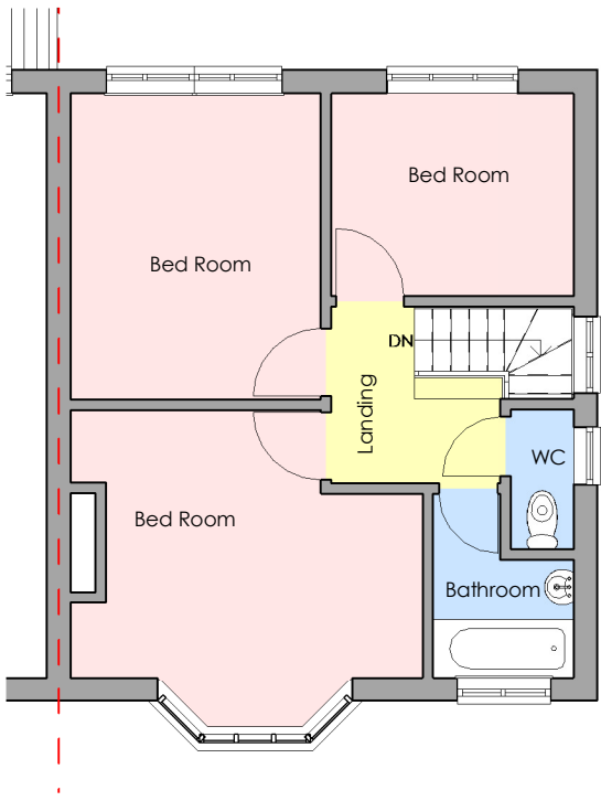
2 Existing First Floor 2553-A-100 1 : 100
