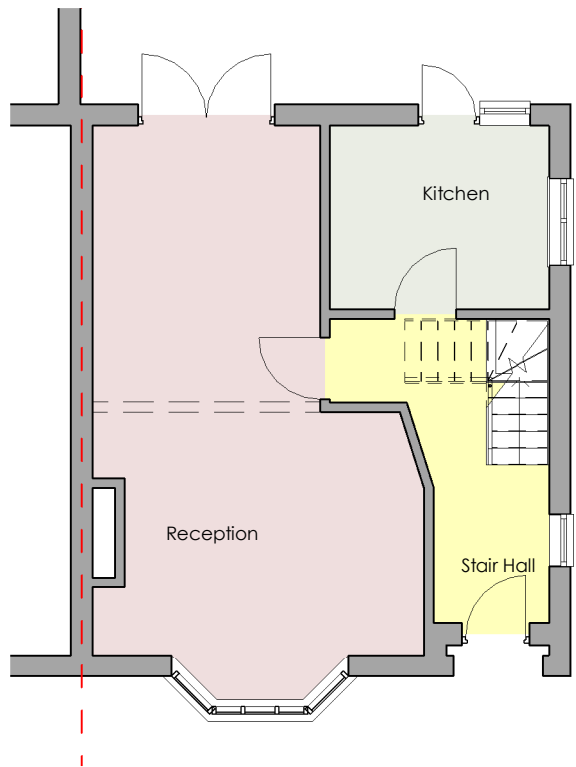
1 Existing Ground Floor 2553-A-100 1 : 100
