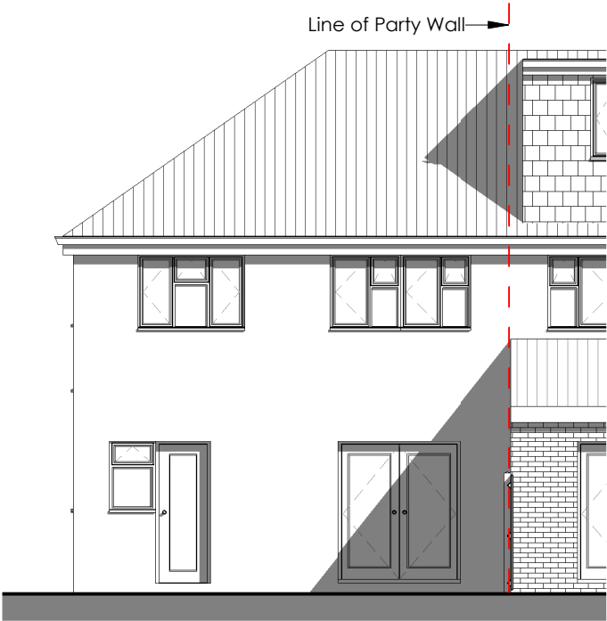
5 Existing Rear Elevation 2553-A-100 1 : 100
