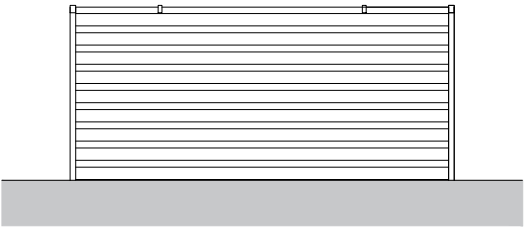
Front 1:100
