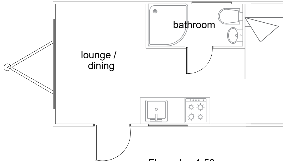
Floor plan 1:50
