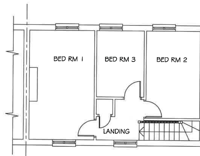
EXISTING FIRST FLOOR PLAN SCALE= 1:100
