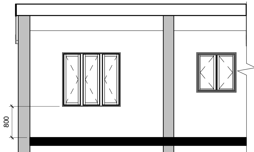
1 A-A First Floor Bedroom Section 1 : 50
