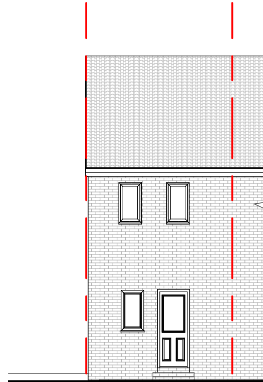
2 Rear Elevation (North) 1 : 100
