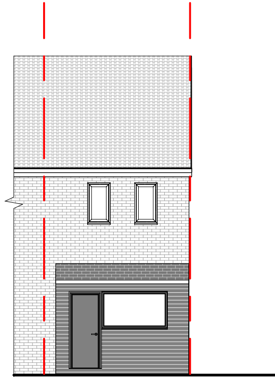
1 Front Elevation (South) 1 : 100
