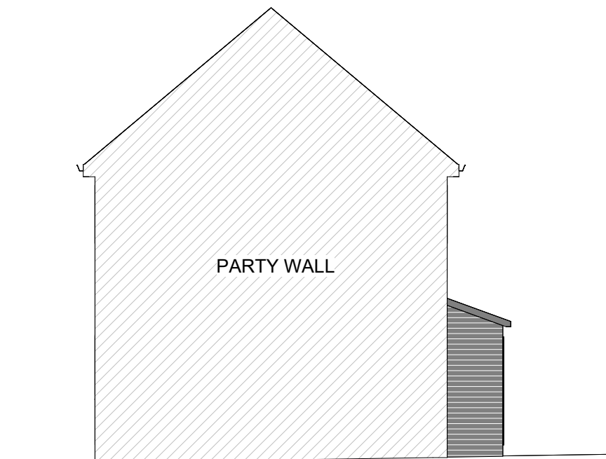
4 Flank Elevation (West) 1 : 100
