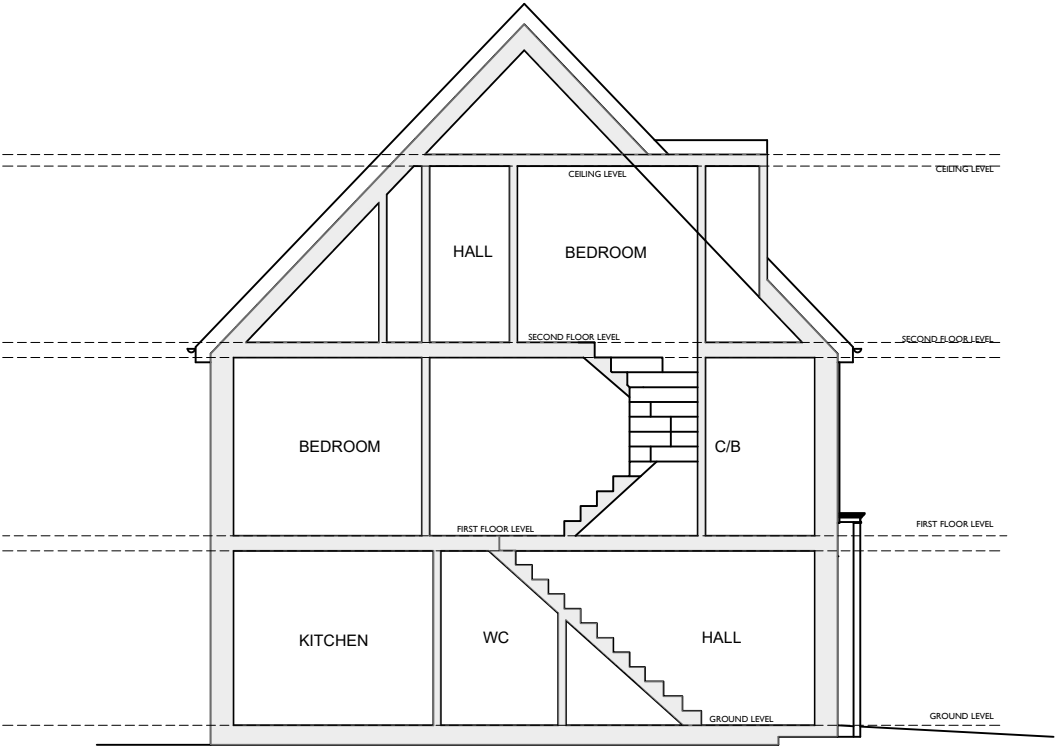
EXISTING SIDE SECTION
