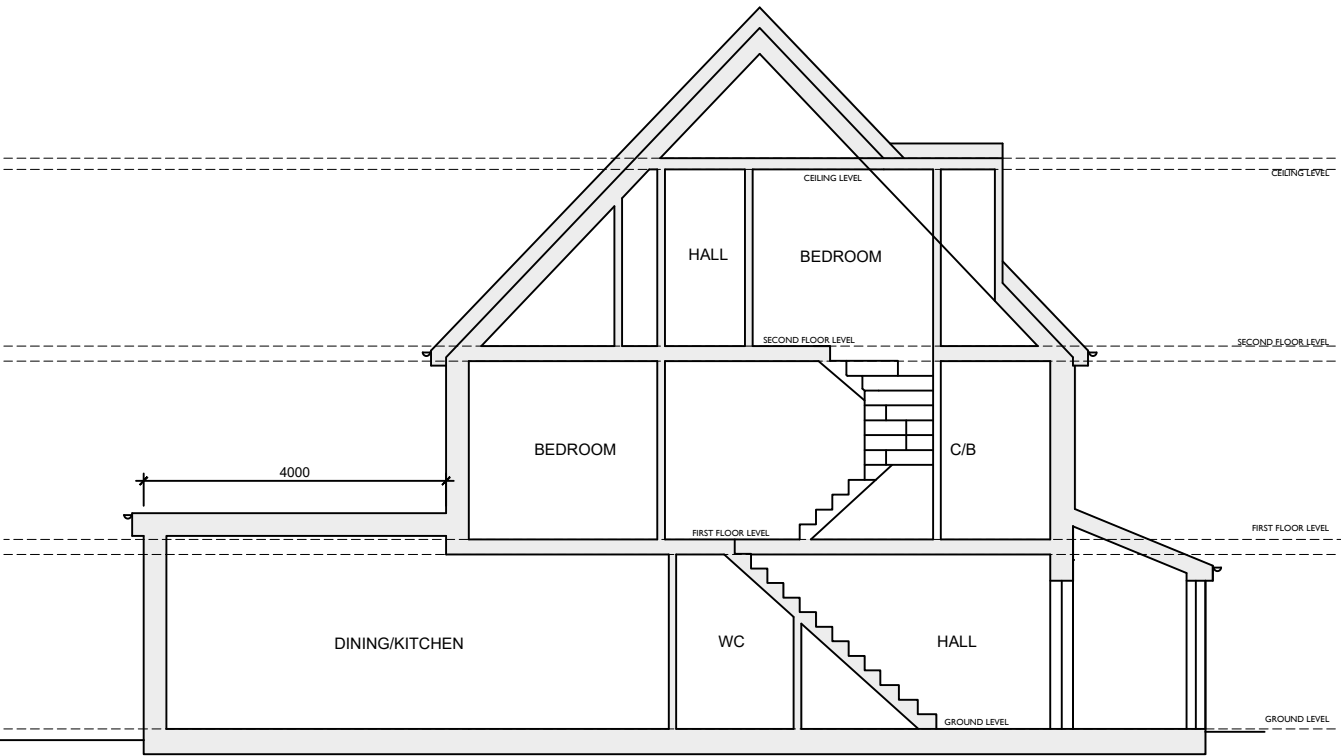
PROPOSED SIDE SECTION
