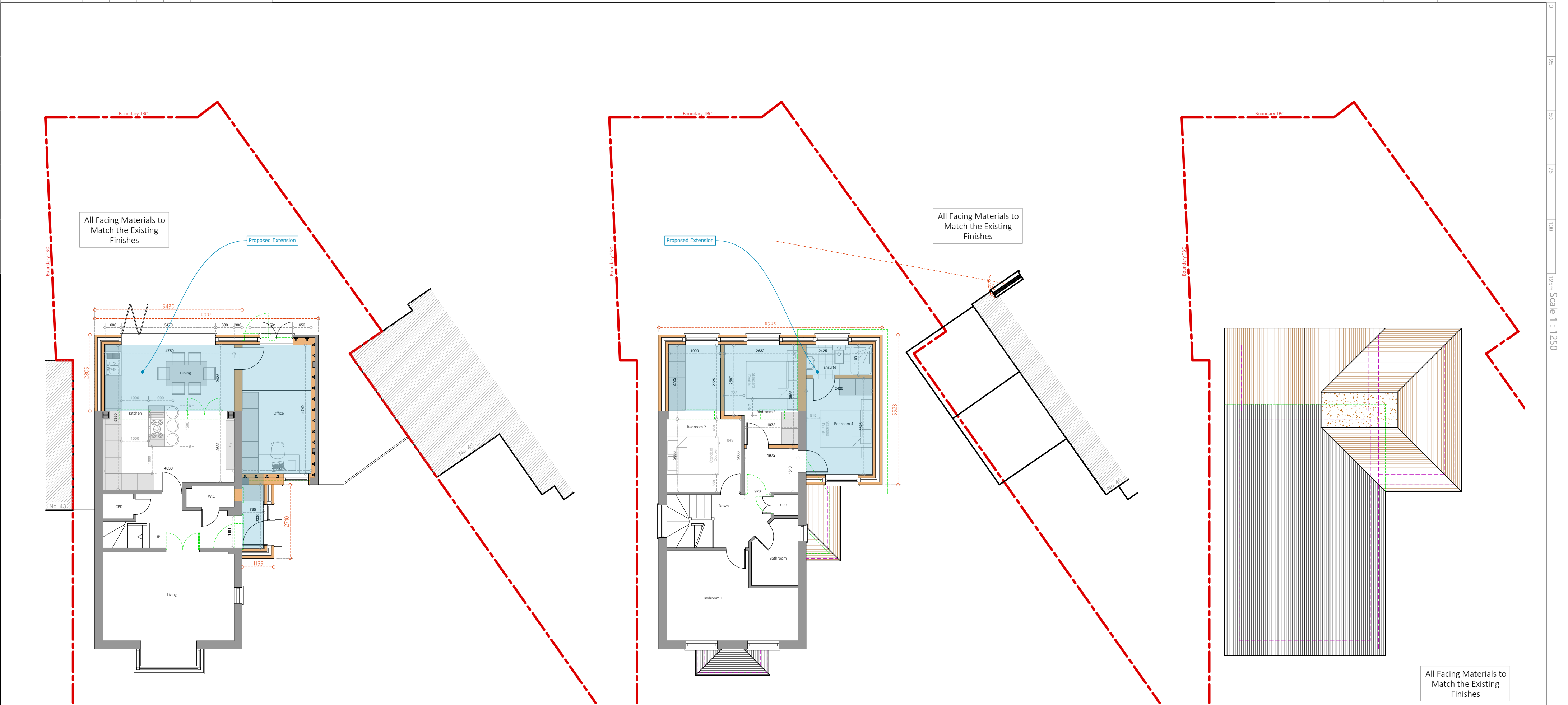
1 Proposed Ground Floor Plan Scale 1/100 2 Proposed First Floor Plan Scale 1/100 3 Proposed Roof Plan Scale 1/100
