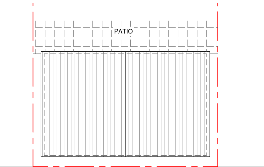
NO.79 PROPOSED OUTBUILDING ROOF PLAN
