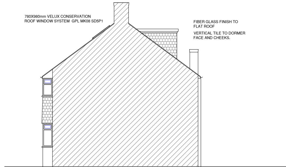
NO.79 PROPOSED SIDE ELEVATION
