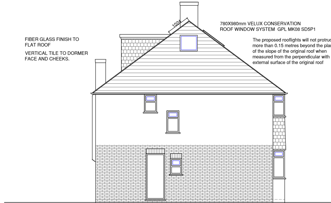
NO.79 PROPOSED SIDE ELEVATION
