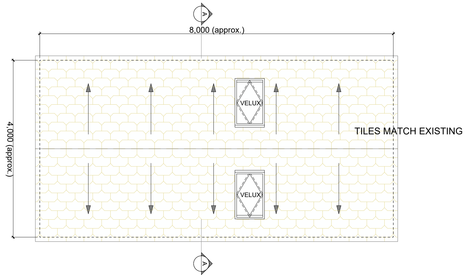
PROPOSED ROOF PLAN SCALE 1:50
