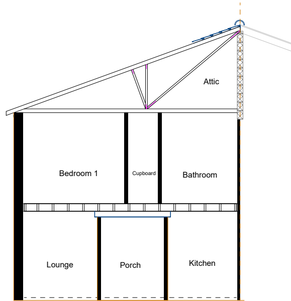
Existing Section
