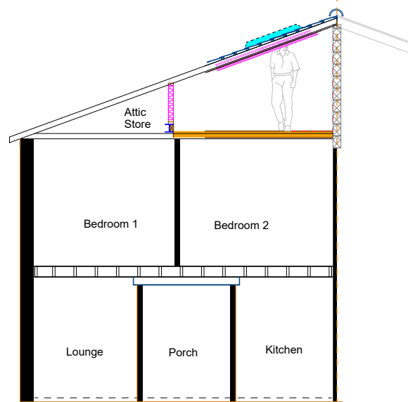
Proposed Section
