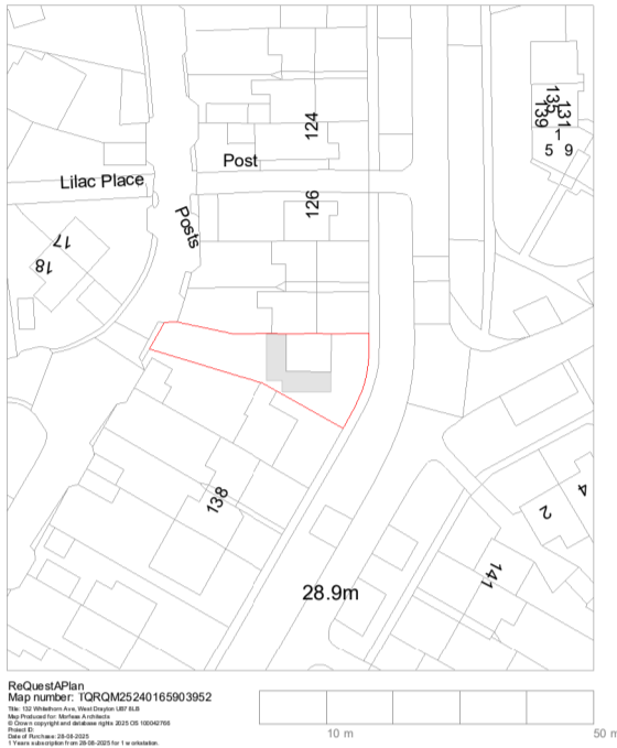
location map 1 : 1250
