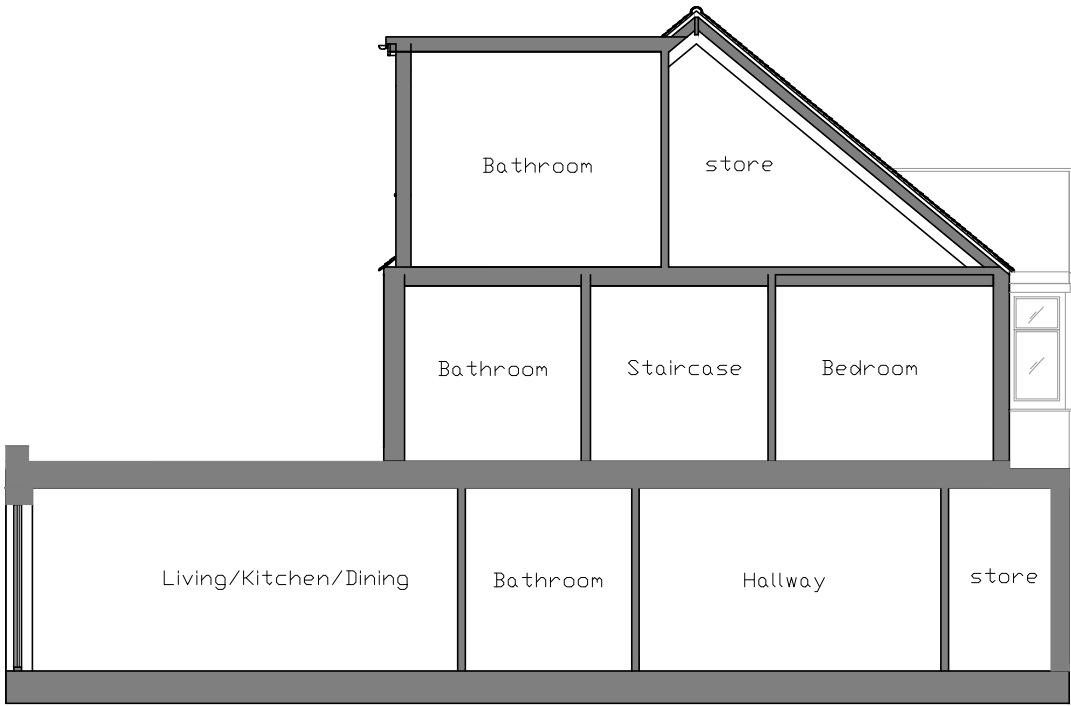
A-A PROPOSED SECTION A-A Scale 1:100 @ A3
