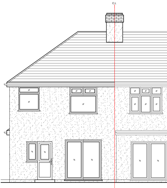
05 - REAR ELEVATION
