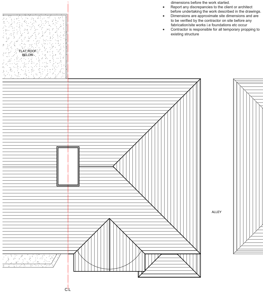
03 - ROOF PLAN
