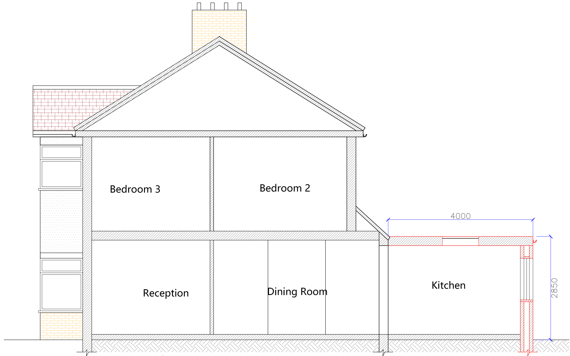
Proposed Section x-x
