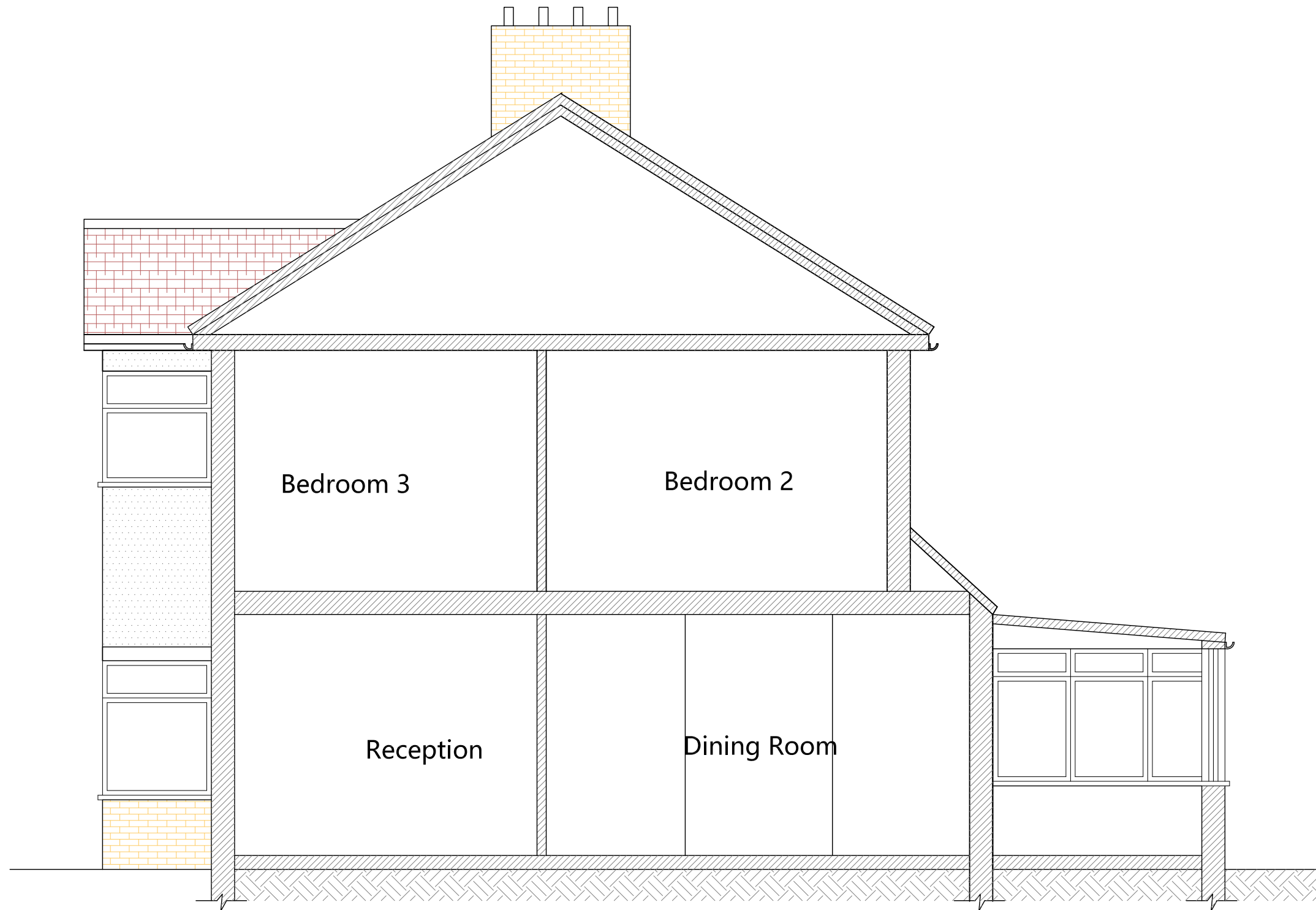
Existing Section x-x
