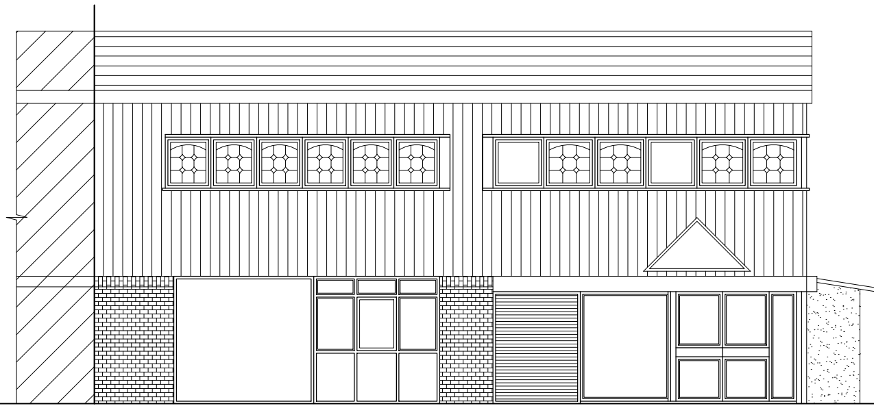
PRE-EXISTING FRONT ELEVATION (1:100 @ A3)
