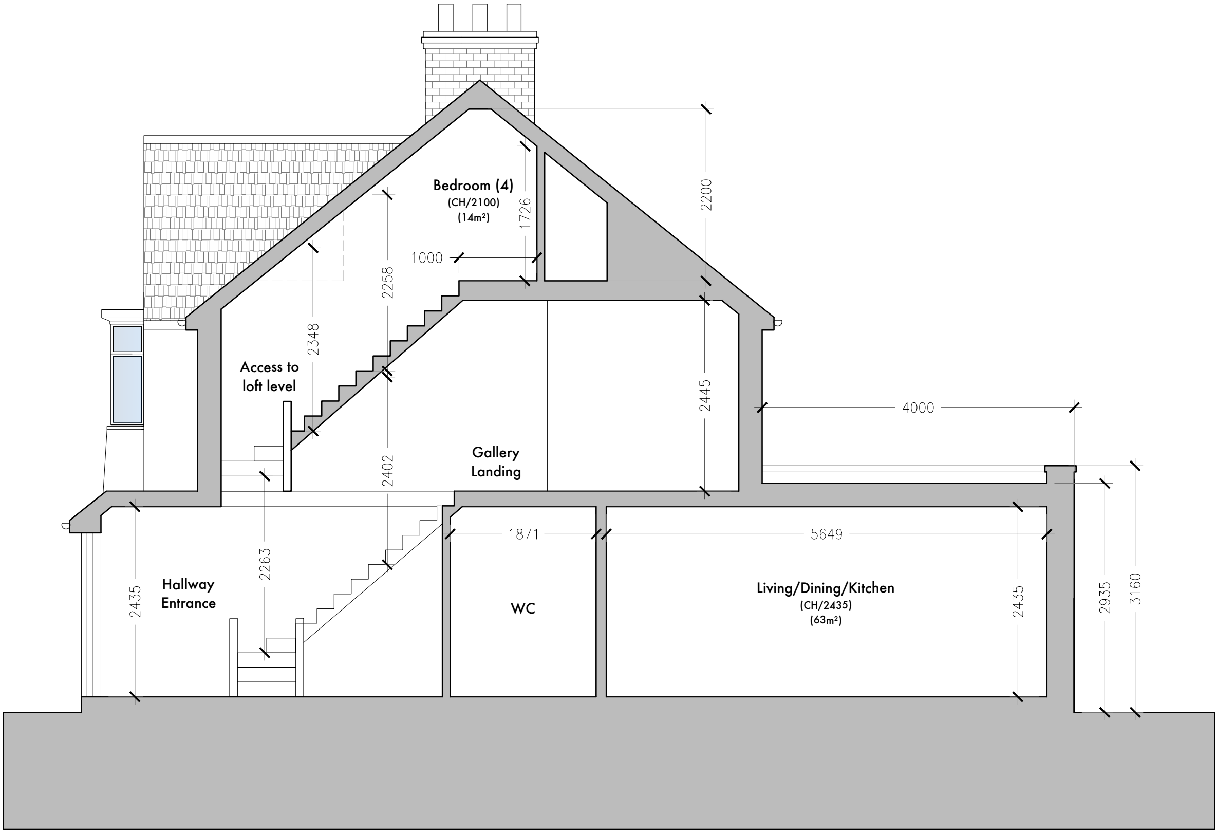
Proposed Section A-A Scale 1:100
