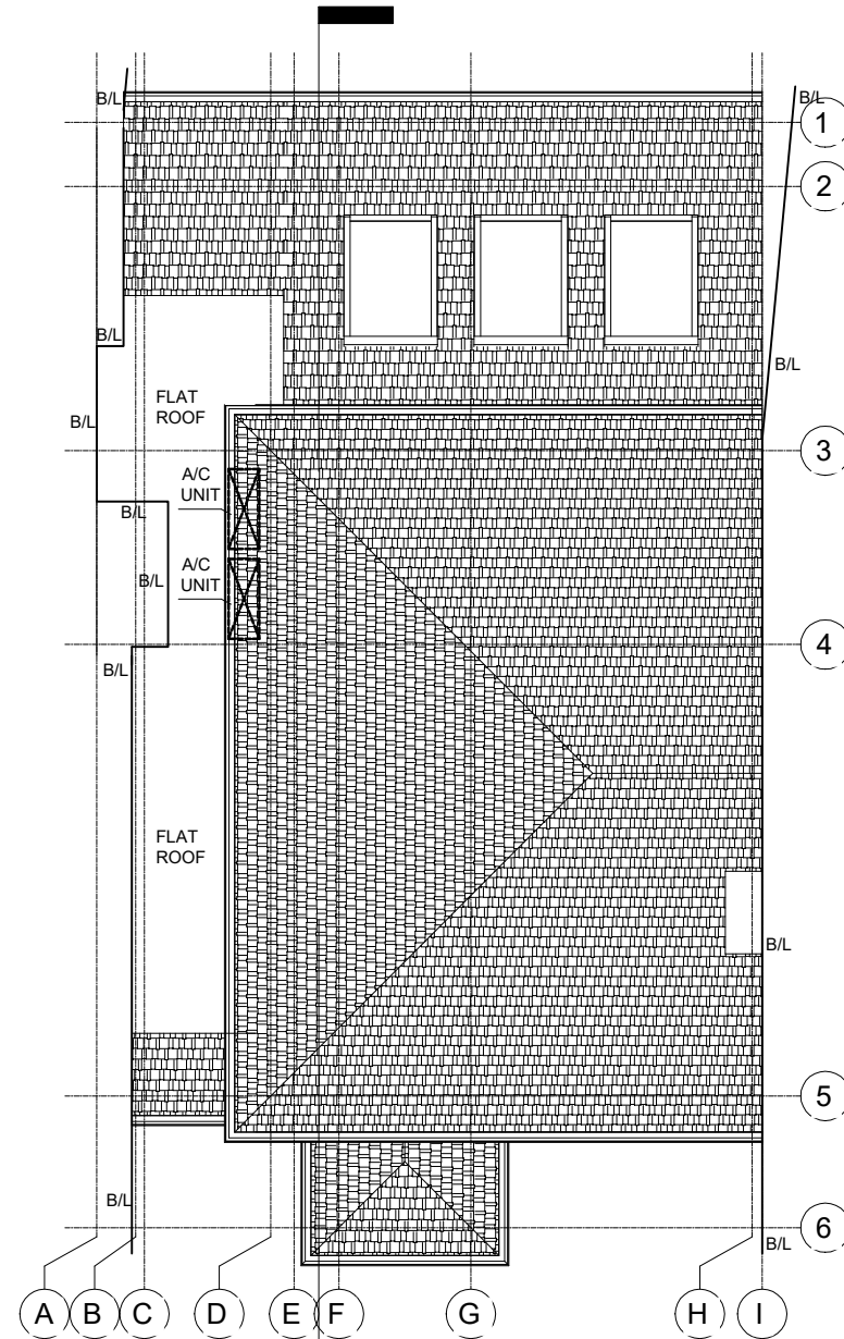
PROPOSED ROOF
