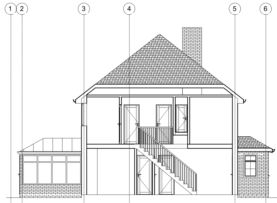
EXISTING SECTION
