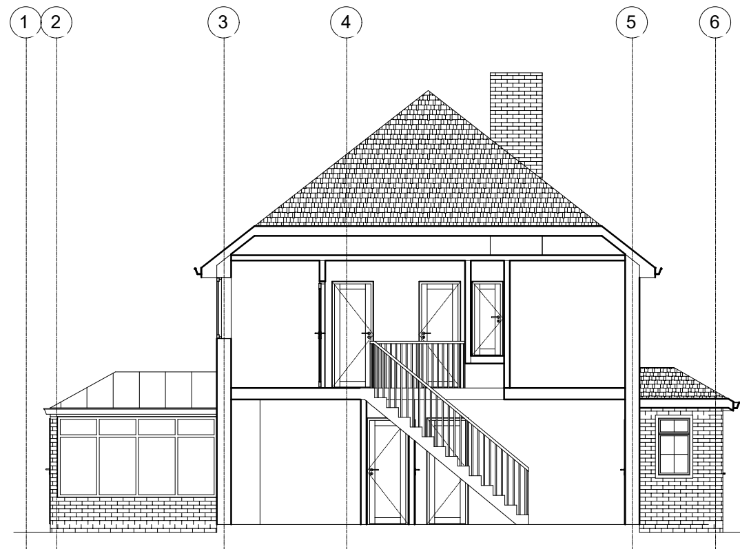
EXISTING SECTION
